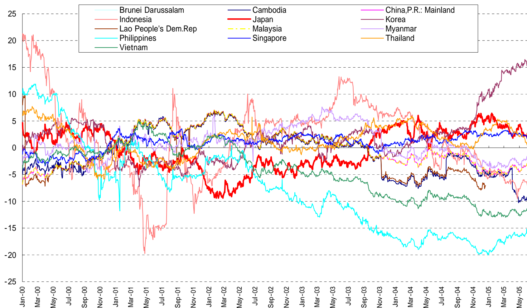
Figure 3. Nominal AMU Deviation Indicators (benchmark year=2000/2001, daily)
